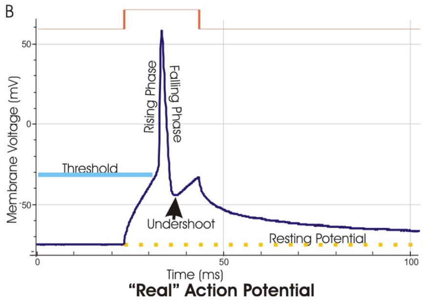
Figure 29 Electrical characteristics of a neurochemical action potential.
